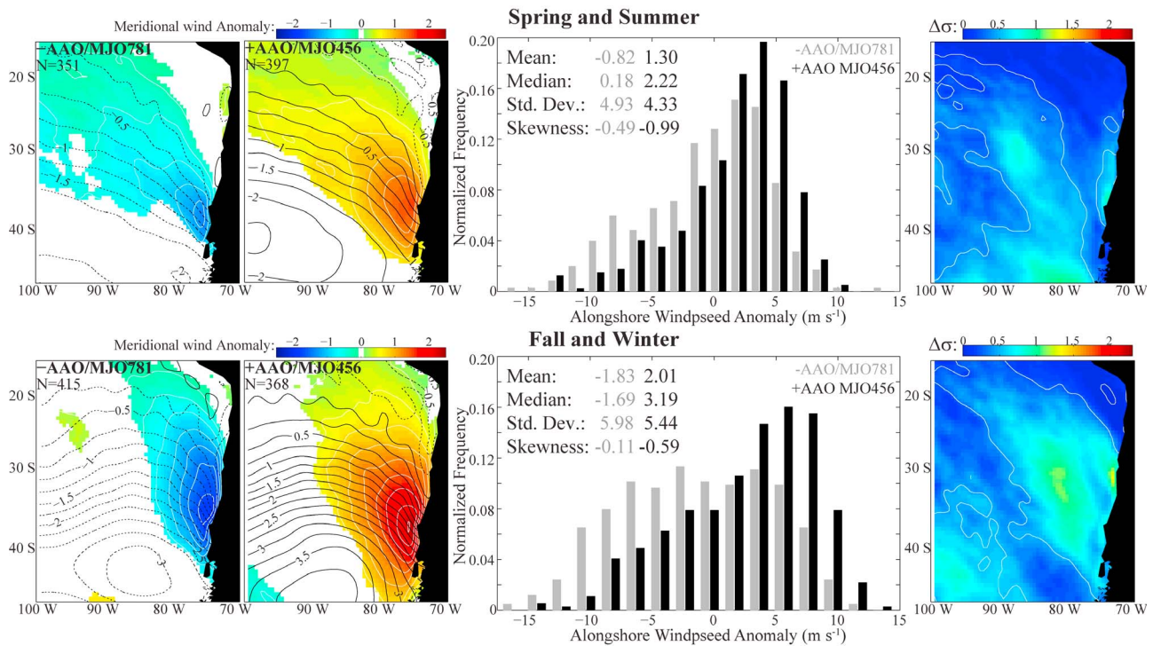
Figure 7. As Figure 3, but for AAO/MJO.
