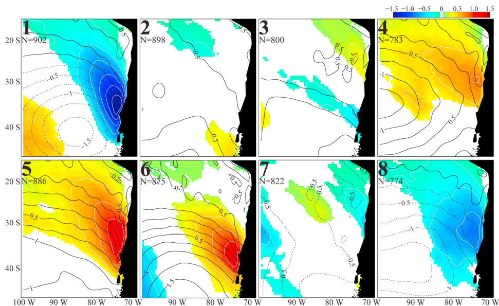
Figure 5. Composites of SLP anomalies (hPa, black contours) and significant meridional wind anomalies ( m s^{-1} , color and white contours every 0.25 m s^{-1} ) binned according to the phase of the MJO that is indicated in each panel. N is the number of days in each composite.
