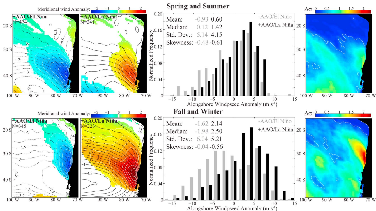
Figure 9. As Figure 3, but for AAO/ENSO.
