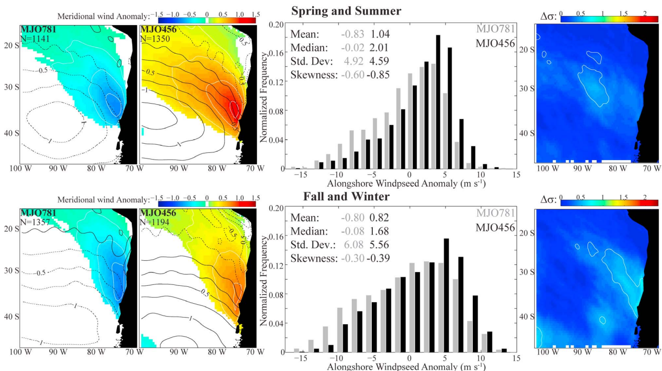
Figure 6. As Figure 3 but for MJO.
